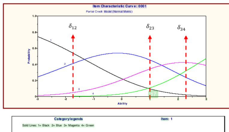
Figure 2. Graph of CRF for item number 1
