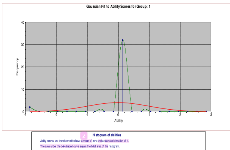
Figure 1. Graph of CRF Estimation of Students' Ability
